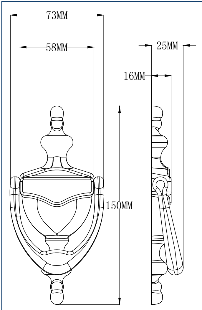
STANDARD URN KNOCKER
