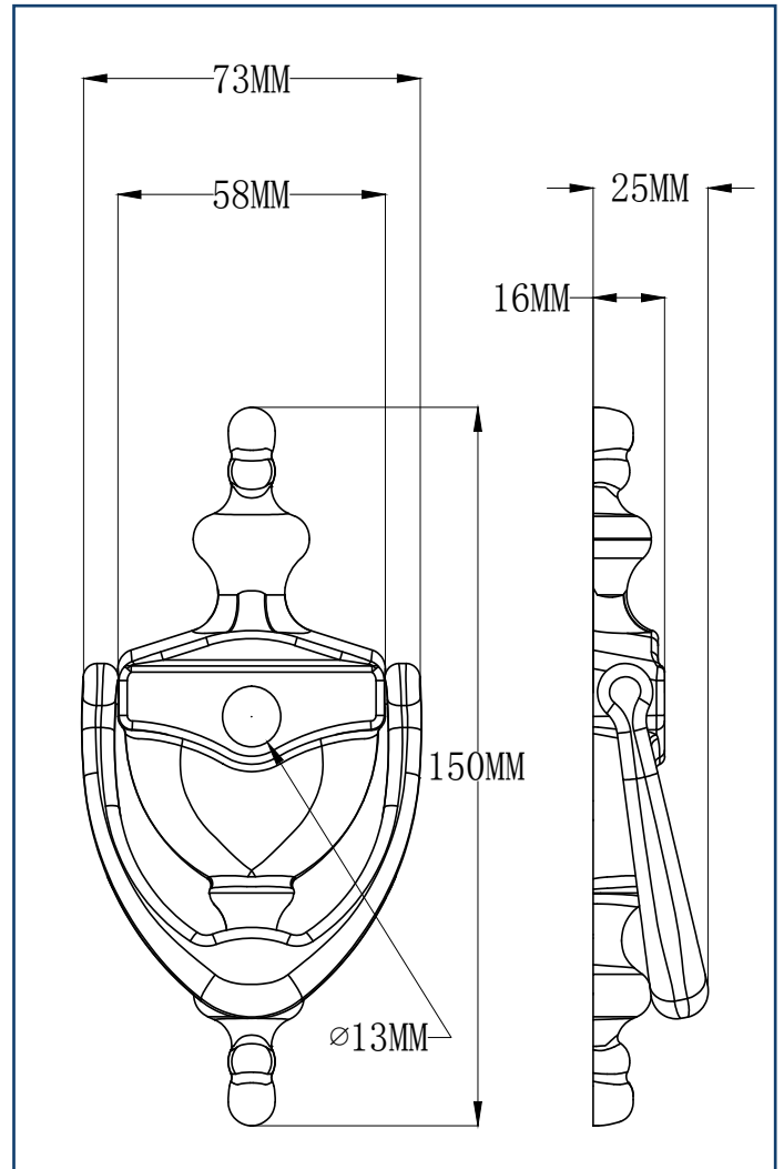
STANDARD URN KNOCKER WITH SPYHOLE
