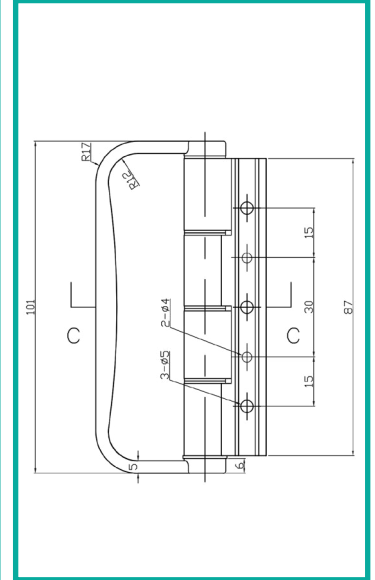
SMARTS HINGE WITH PULL
