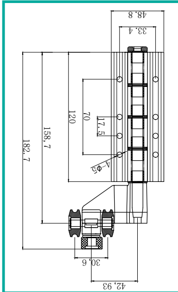
ALUK BOTTOM ROLLER
