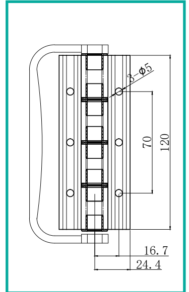
ALUK HINGE WITH PULL
